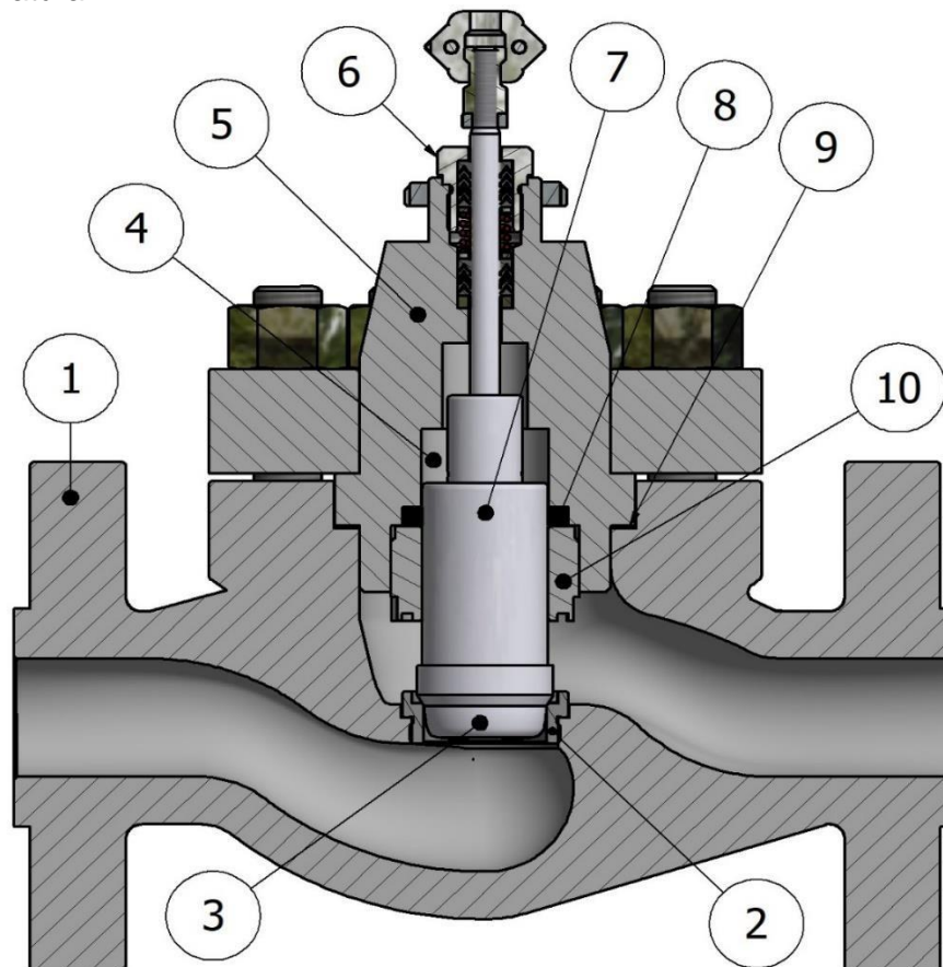
VALVOLA STANDARD
